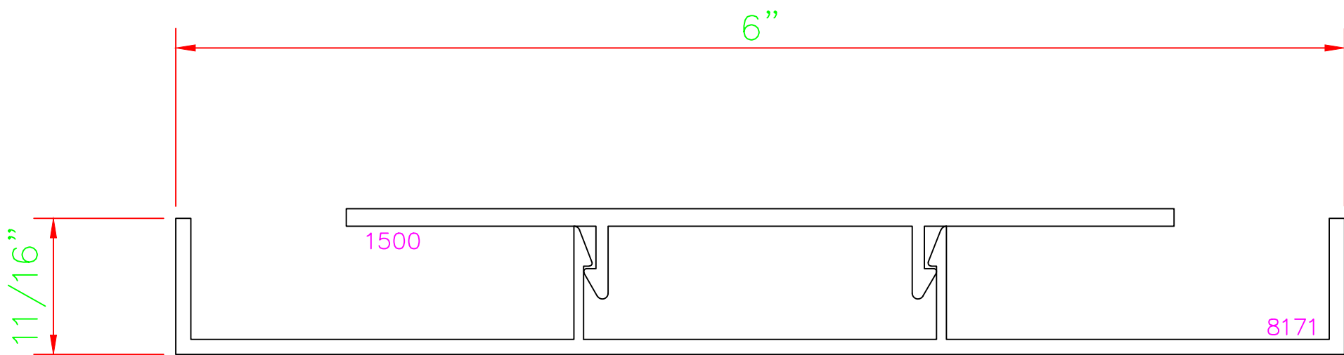
8171 / 1500 6" X 11/16" SNAP TRIM & CLIP
